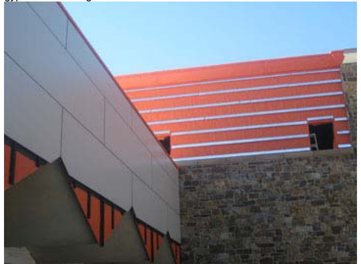
Horizontal Z girts installed (background) over the WrapShield SA Self-Adhered (orange)
