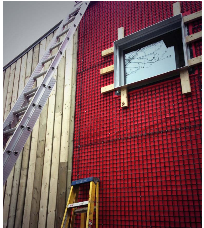
Both WrapShield Water Resistive Vapor Permeable Air Barrier and SlopeShield Water Resistive Roof Underlayment were used on the renovation project.
