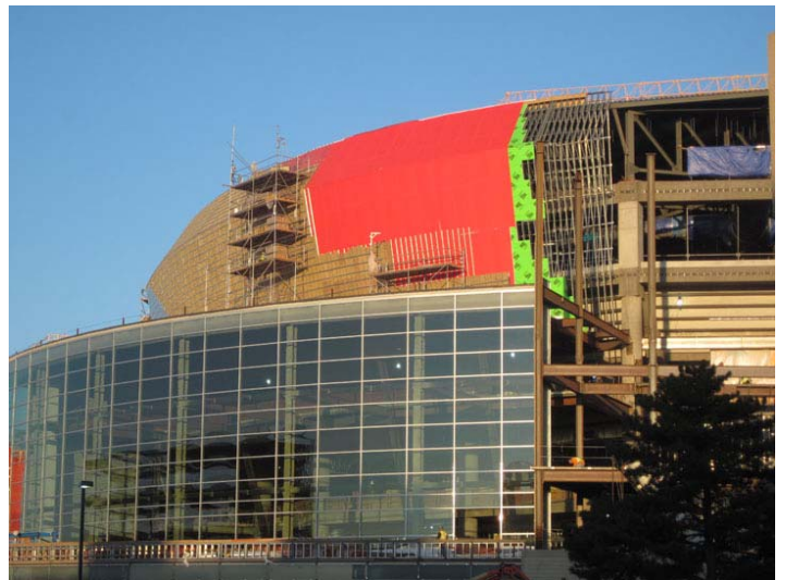
Over 150,000 sq.ft. of WrapShield SA Self-Adhered Water Resistive Vapor Permeable Air Barrier Sheet being installed in a special color: red to match Cornhusker red.
