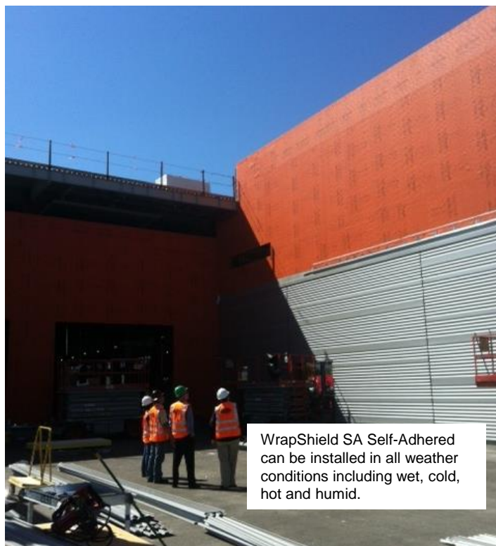
Over 65,000 sq.ft. of WrapShield SA Self-Adhered Water Resistive Vapor Permeable Air Barrier was installed on the Pier 27 Cruise Terminal.
