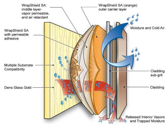
WrapShield SA Self-Adhered Membrane Construction.
