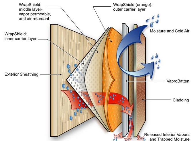
WrapShield SA Self-Adhered Membrane Construction.
