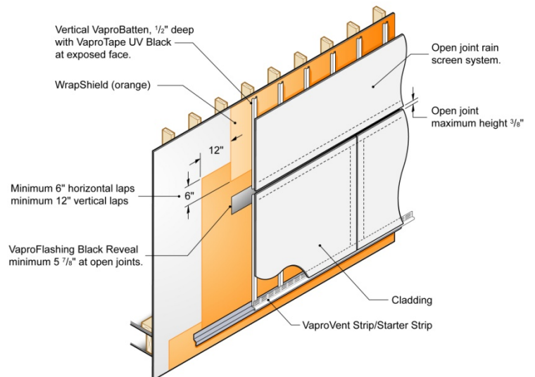
Application drawing of WrapShield with VaproFlashing Black under open joint rain screen cladding system
