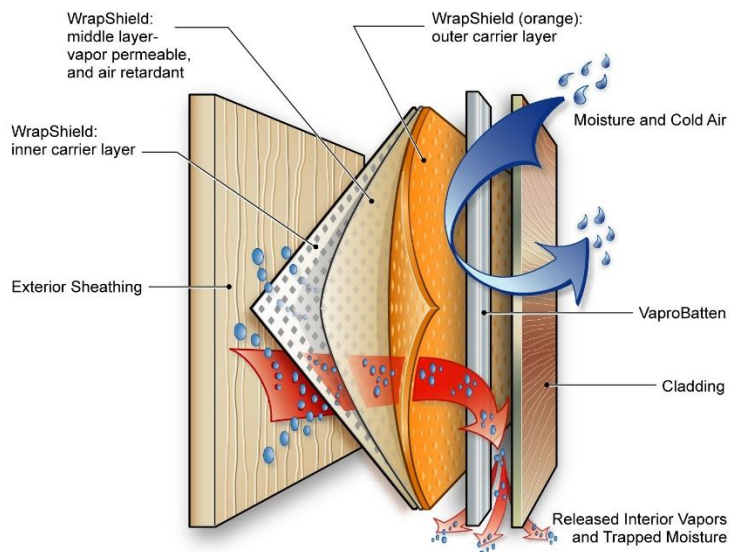
WrapShield construction.
