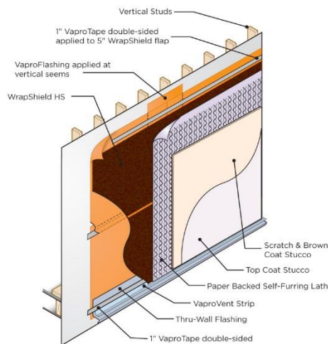
WrapShield HS Lap detail for Typical Stucco Assembly
