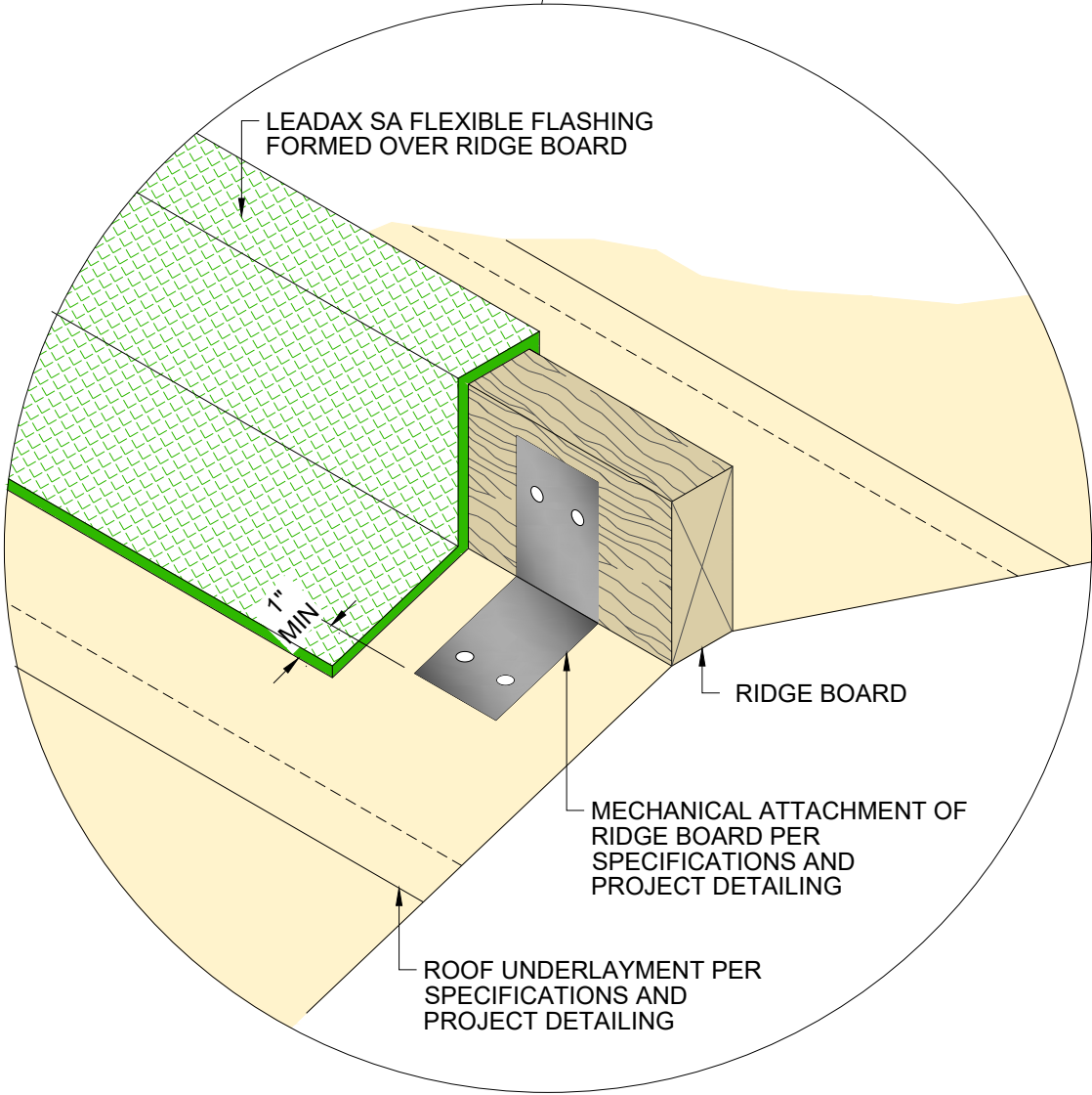
HIP / RIDGE SUPPORT DETAIL
