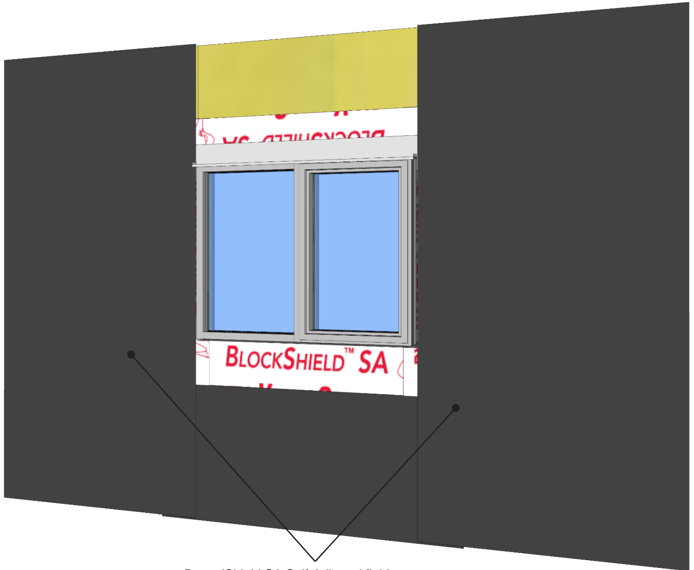
RevealShield SA Self-Adhered field membrane installed vertically with minimum 3" overlap,
