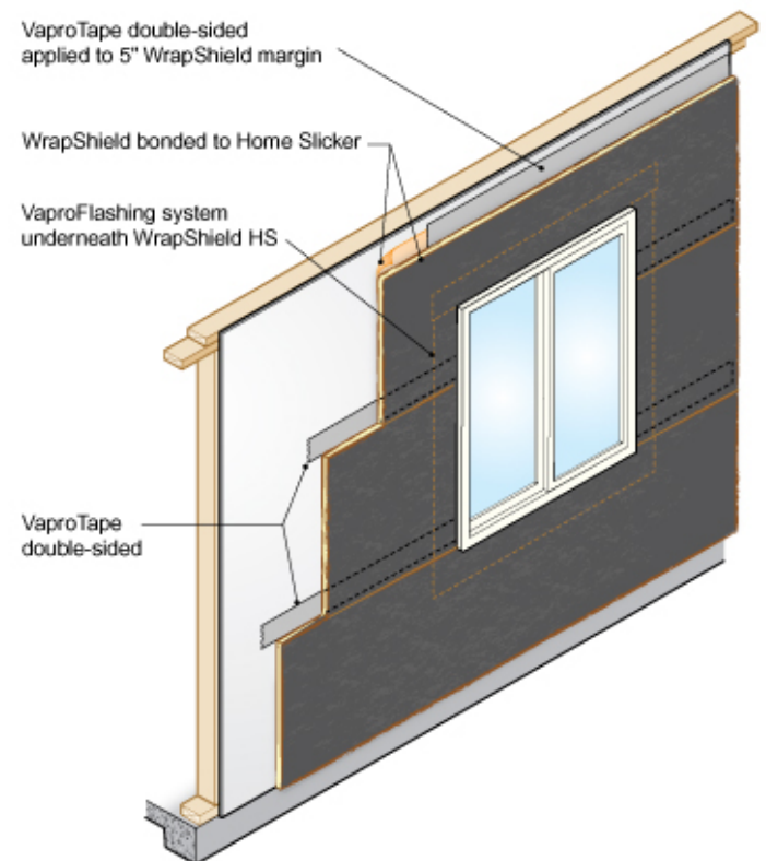
WrapShield HS detail showing application (above); closeup photo showing tight and "clean" application (left).
