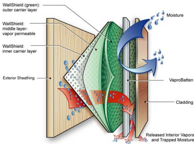
WallShield membrane construction
